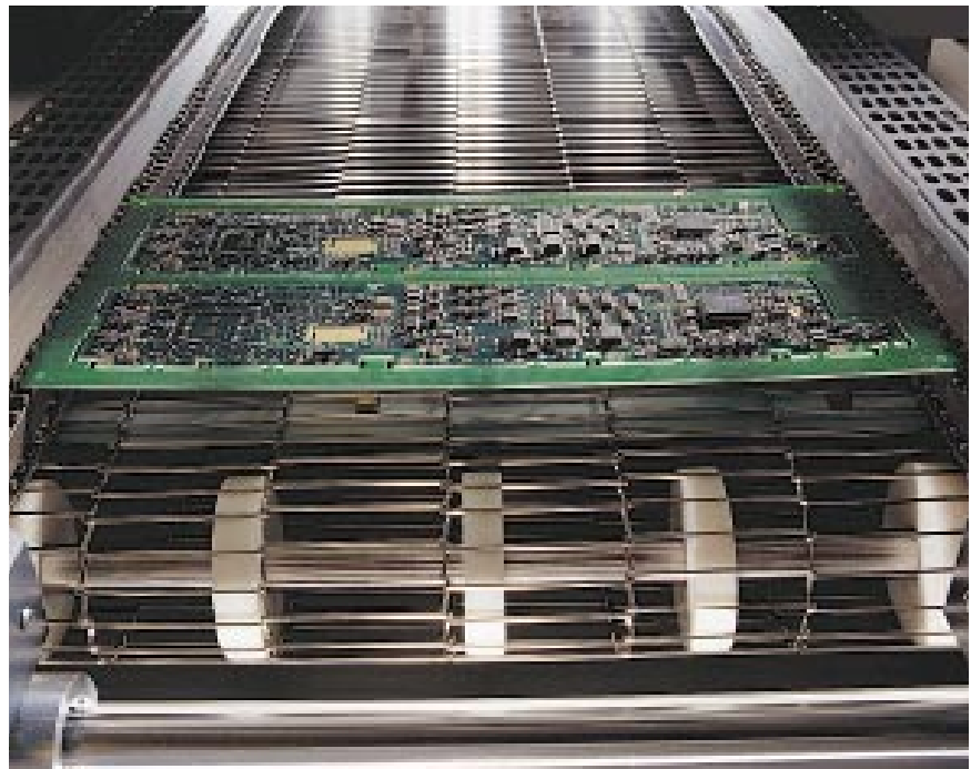
All full convection reflow ovens are engineered to handle the special requirements of double-sided PCBs.
