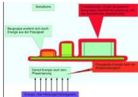
Image 2 Energy flow in a vapor phase
